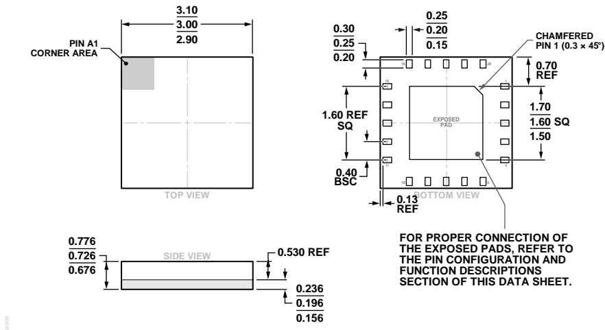
Figure 24. 20-Terminal Land Grid Array [LGA] 3 mm x 3 mm Body and 0.72 mm Package Height (CC-20-3) Dimensions shown in millimeters
